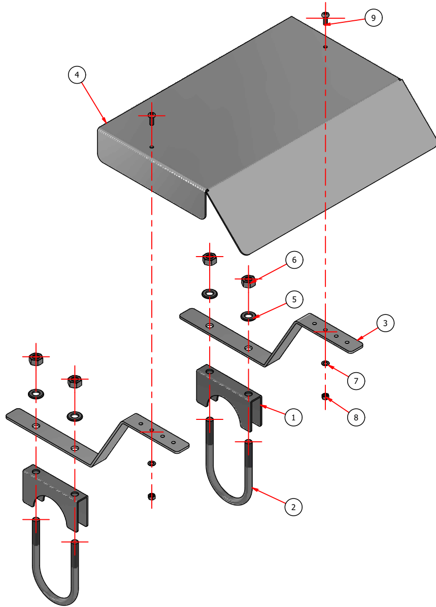
VISTA EXPLODIDA ( 1:5 )
